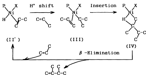
Fig. 15. Estimated mechanism of propylene dimerization.
